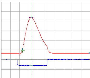
Output signals: Amplitude, NIM-Trigger, Y=1V, X= 500ns
